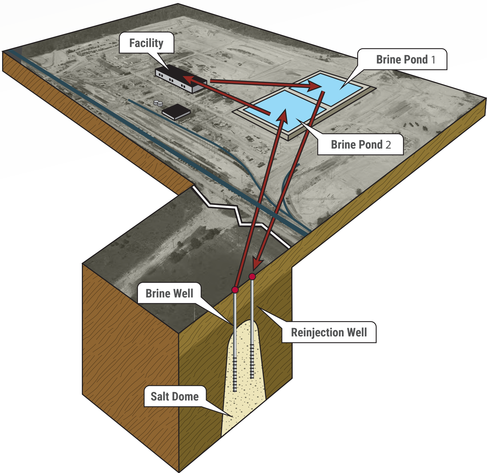
Process Water Flow Diagram
